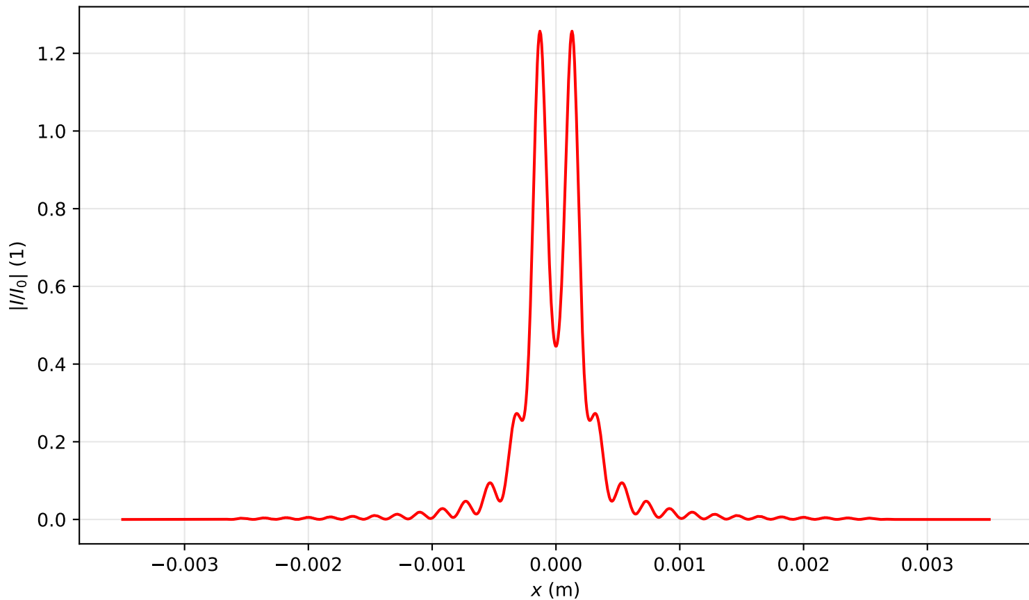
Intensity profile I(x, y = 0, z = 0.159)/I_0 , P_{in}=5.0P_{cr} , artificial time
